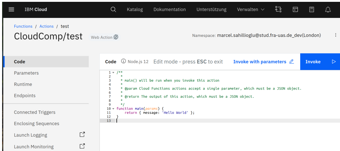
Figure 2: Development Environment
