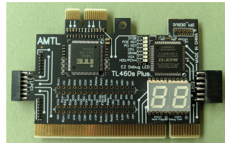
POST card for PCI, PCIe and LPC Bildquelle: Markus Kuhn. Wikimedia (CC0)
